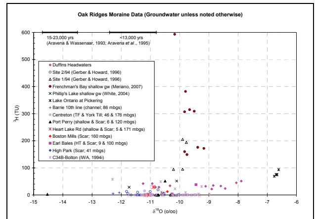
Figure 8: Tritium versus \delta^{18}\text{O} for select samples.
