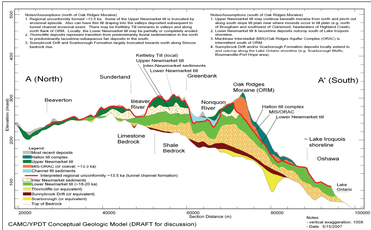
Figure 3: North-south cross section. See Figure 2 for section location.
