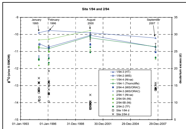
Figure 7: Site 1/94 and 2/94 \delta^{18}\text{O} and d versus time.
