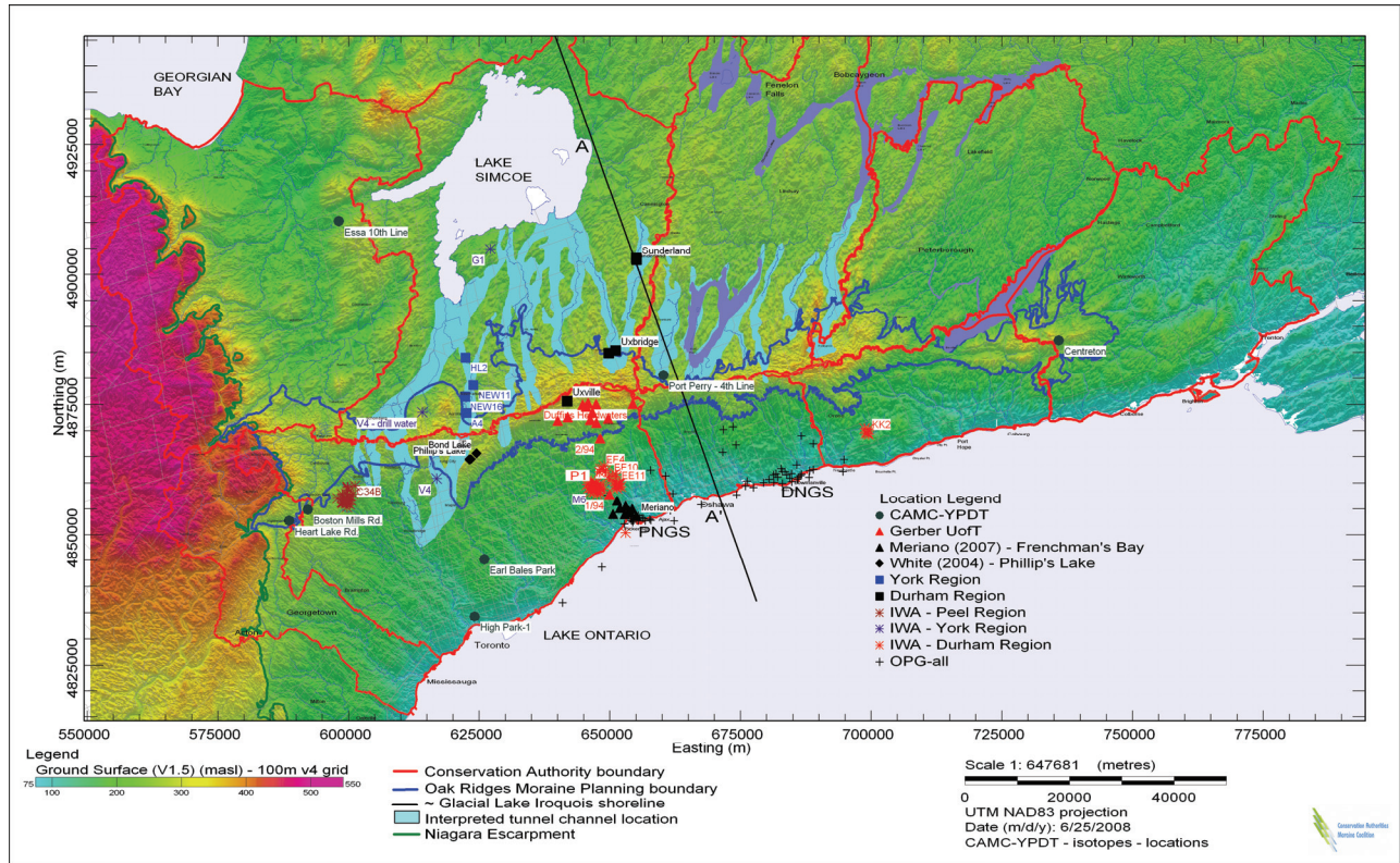
Figure 2: Study area showing ground surface topography, sample locations and cross section location
