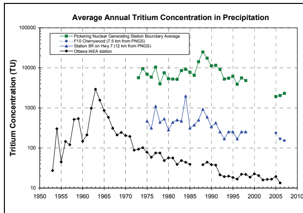
Figure 4: Measured tritium concentration in precipitation.
